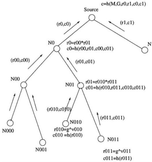
Fig. 1. Computation of the Merkle Tree
