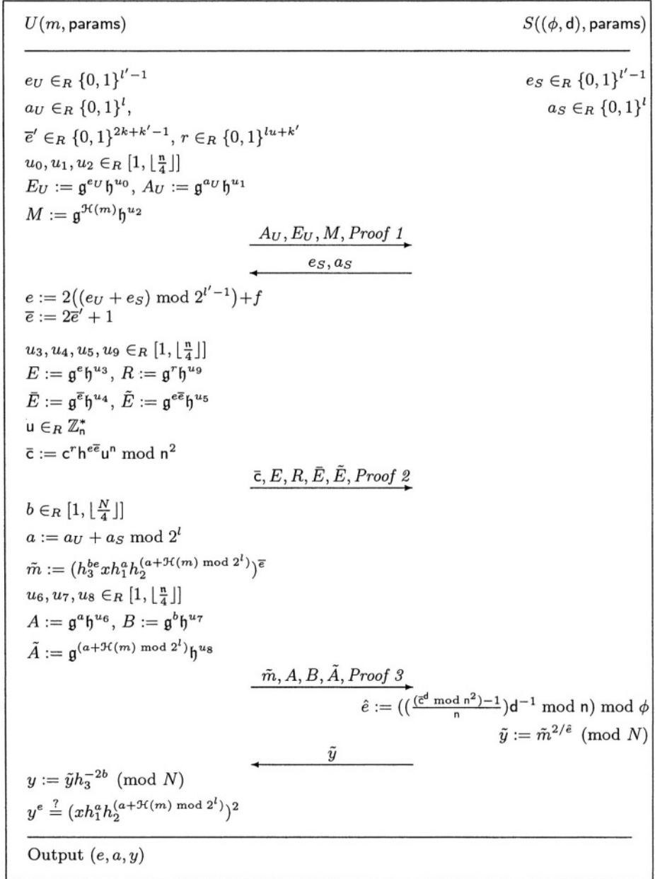
Fig. 1. A two-party protocol for producing mCSF signatures. The signer does not learn any information about the signed message. Here, the common parameters params are ((N, h_1, h_2, h_3, x, f, n, h, g, n, c, h, k, k', l, l', u))
