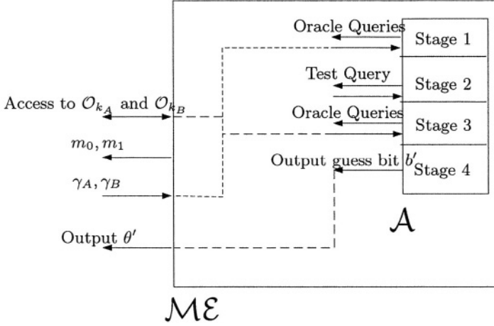
Fig. 5. Game \mathcal{G}_{\mathcal{ME}}
