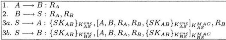
Fig. 4. An improved provably secure 3PKD protocol
