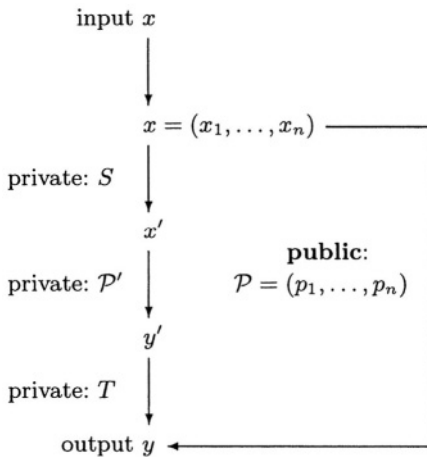
Fig. 2. MQ-trapdoor (S, \mathcal{P}', T) in STS
