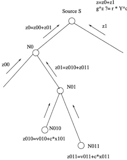
Fig. 3. Default propagation of the responses z_i
