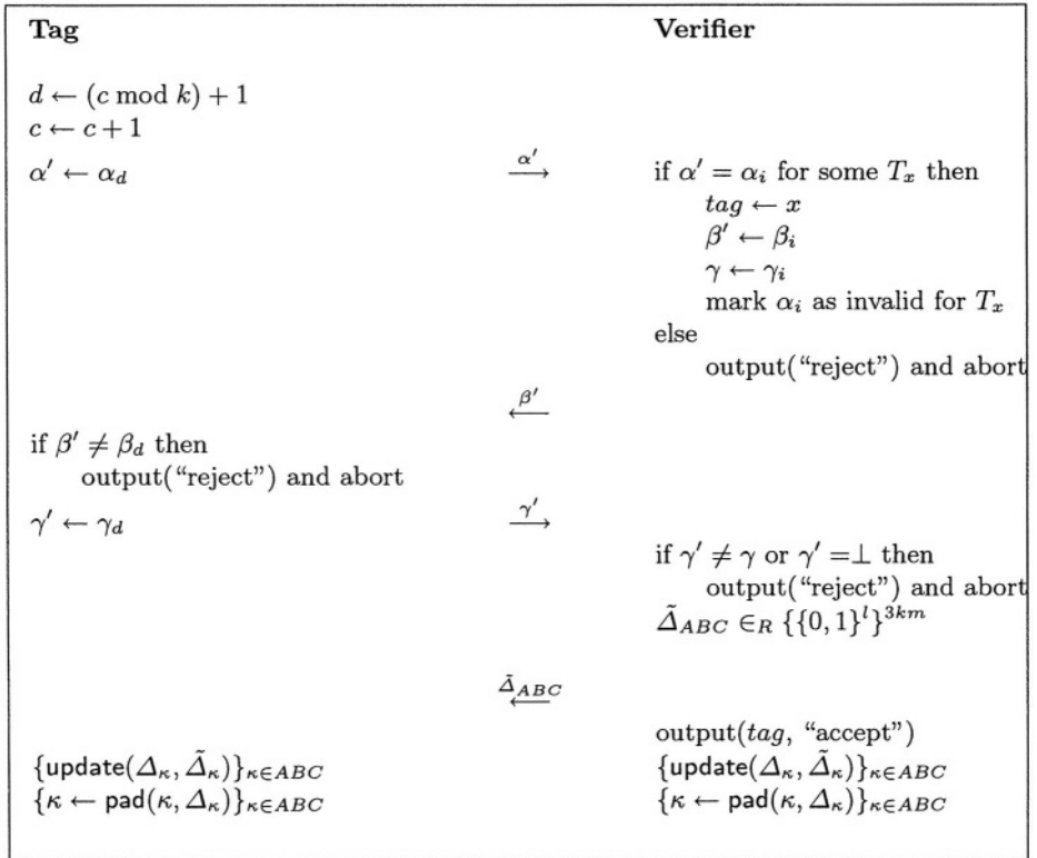
Fig. 1. Full RFID-tag authentication protocol
